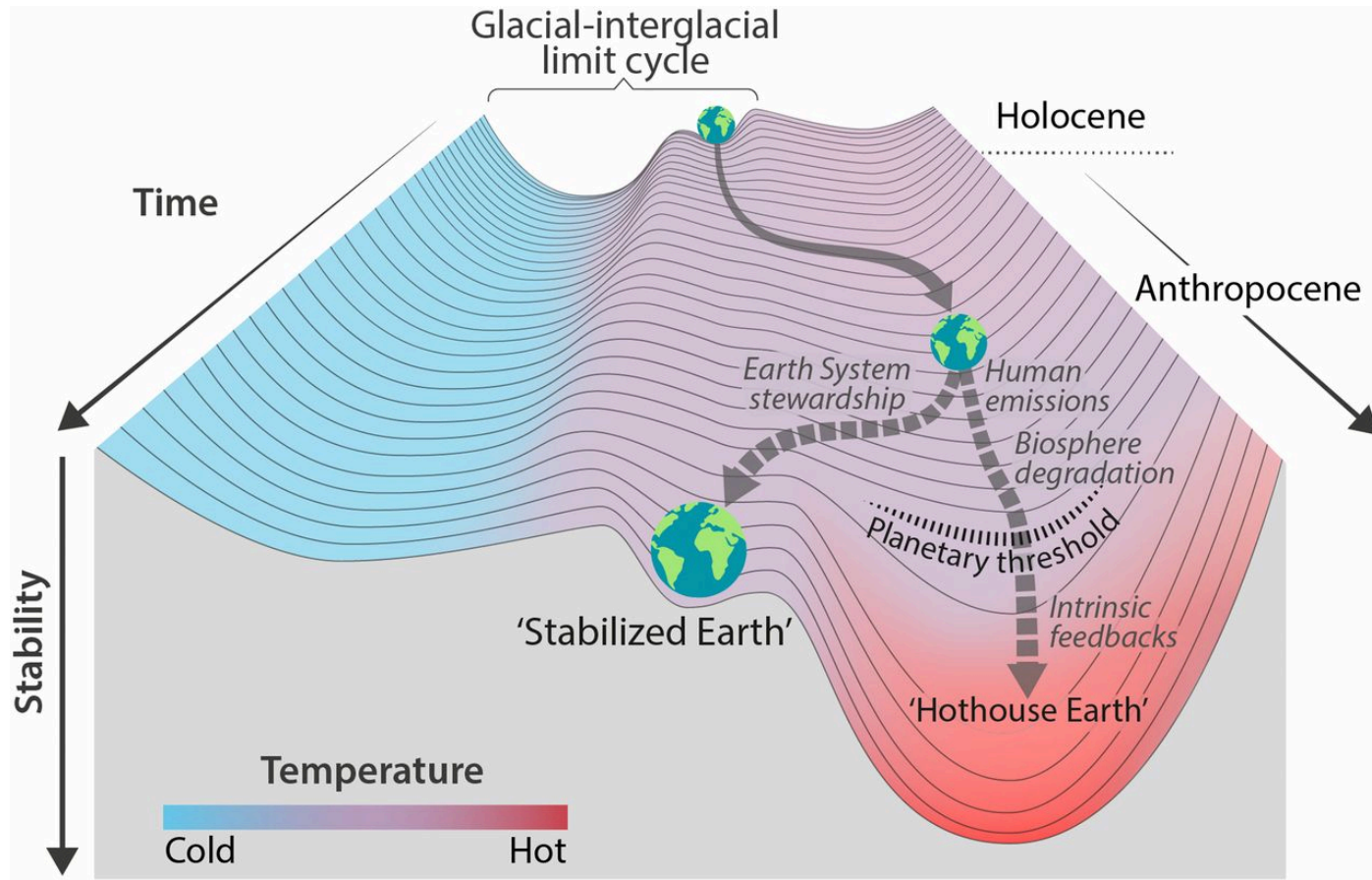
Trajectories of the Earth System in the Anthropocene (Hothouse Earth Report)
